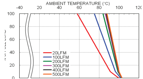
LPB30-48S5 Derating Curve With Heat-sink
