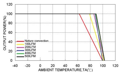
LWB40-24S05 Derating Curve
