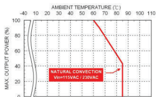
Derating Curve vs. Ambient Temperature KUI30-xxB xx=33, 5, 75, 9, 121, 151, 18 Connector Option: (Blank; JST)
