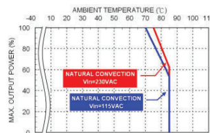
Derating Curve vs. Ambient Temperature KUI30-xxB xx=12, 15, 24, 28, 36, 48, 53 Connector Option: (Blank; JST)
