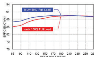
Efficiency vs. Input Voltage KUI30-24SB
