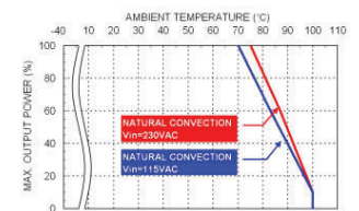
Derating Curve vs. Ambient Temperature KUI30-xxB xx=12, 15, 24, 28, 36, 48, 53 Connector Option: (-M, -T, -D)
