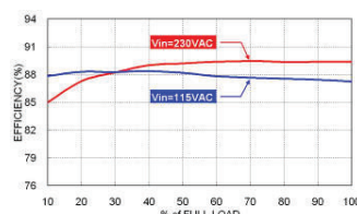
Efficiency vs. Output Load KUI30-24SB
